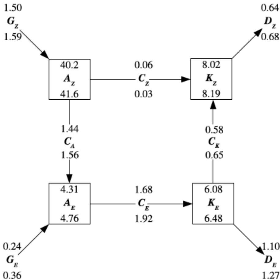
Figure 1. Energy cycle diagram averaged over 1979–2001 for NCEP (top values) and ECMWF (bottom values) Reanalyses. Energy amounts in units of 10^5 J m^{-2} and transformation rates in W m^{-2} .
